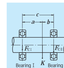
Fig. 5.5 Radial Load Distribution (1)
