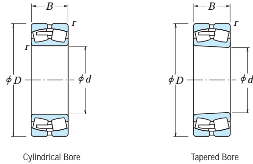
Cylindrical Bore
