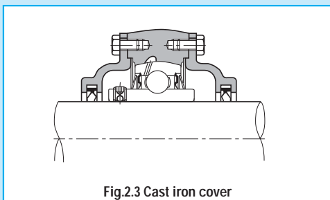
Fig. 2.3 Cast iron cover
